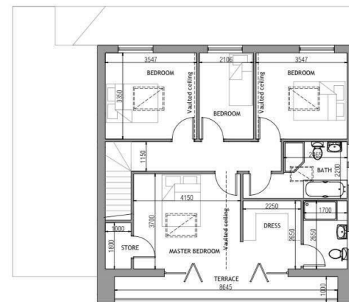
FIRST FLOOR GIA - 78.7m 2
