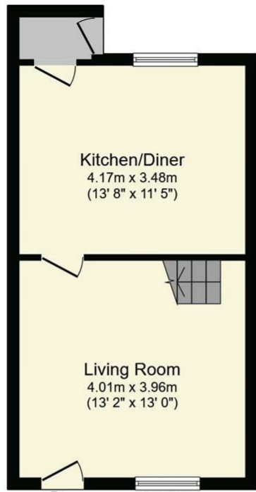
Floor area 32.8 sq.m. (353 sq.ft.) approx
