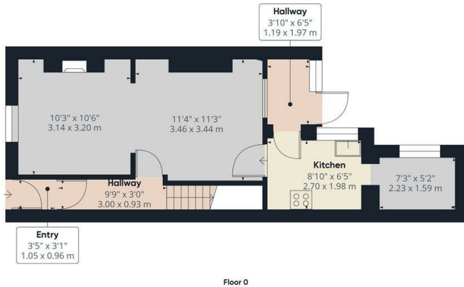
Floor 0
